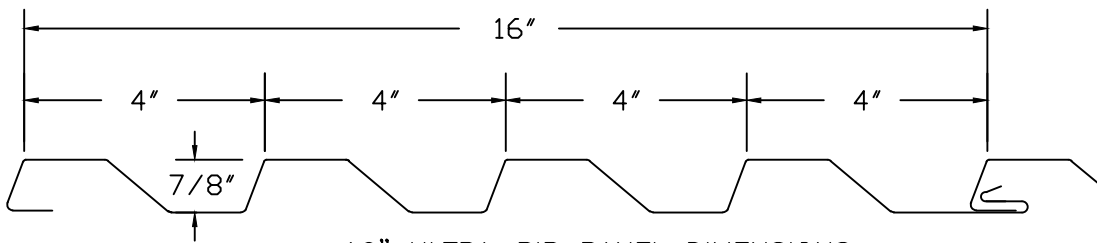
16" ULTRA-RIB PANEL DIMENSIONS
