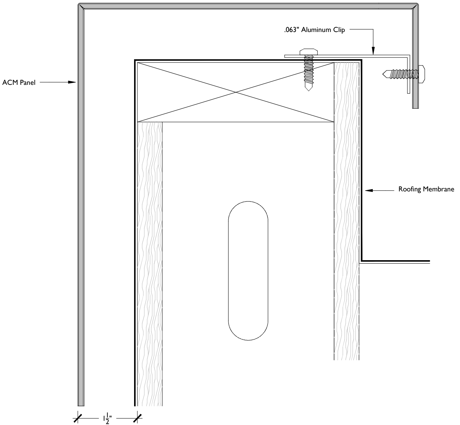
5 Typical Parapet Termination
